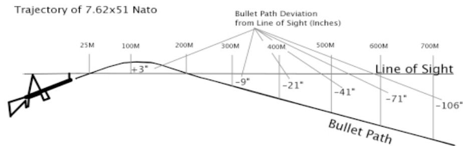
Figure 30. 7.62x51 Ball Trajectory
